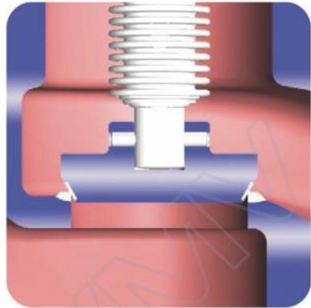
1. Conical sealing surface will remove impurity automatically.
